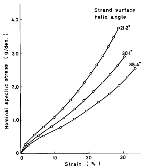
Fig. 3.20. Stress-strain curves of 19-yarn strand at various degrees of twisting.
