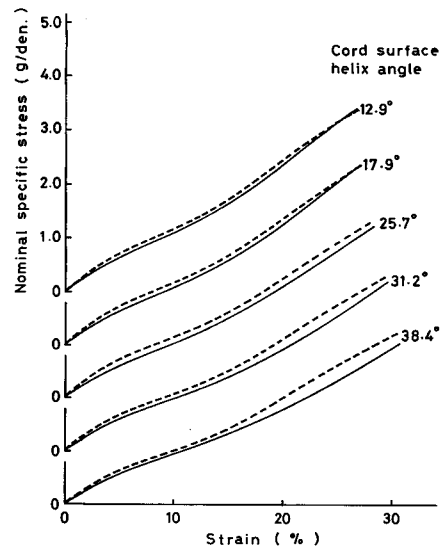
Fig. 4.5. Calculated and experimental stress-strain curves of 3-ply cord single yarn strand of 50 turns per 6 in. lower twist at various degrees of twisting. solid line; experimental, broken line; calculated.
