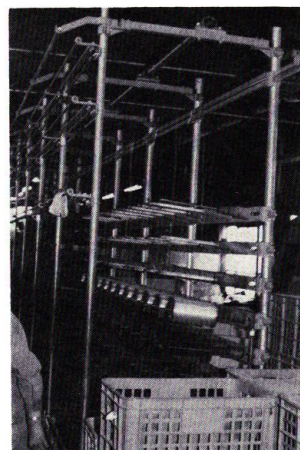
Fig. 3.2. Frame for setting the bobbin of yarn.
