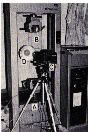
Fig. 3.15. Apparatus for the determination of the change of cord diameter by tension. A; Strength testing machine, B; Test piece, C; Camera, D; Light.
