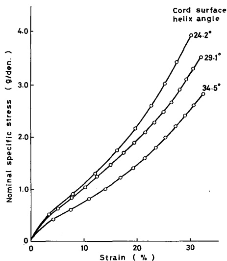
Fig. 3.23. Stress-strain curves of 2-ply cord 3-yarn strand at various degrees of twisting.
