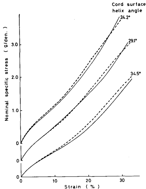
Fig. 4.13. Calculated and experimental stress-strain curves of 2-ply cord 3-yarn strand at various degrees of twisting. solid line; experimental, broken line; calculated.
