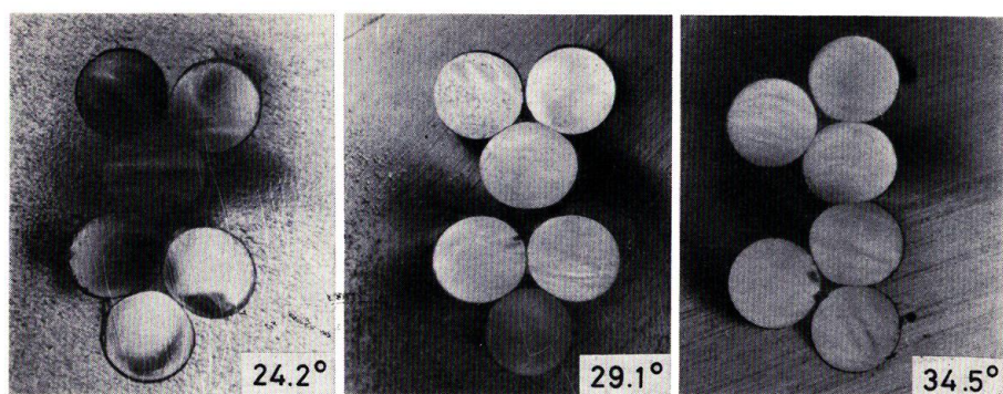
Fig. 3.31. Cross sections of 2-ply cord 3-yarn strand at various surface helix angles.
