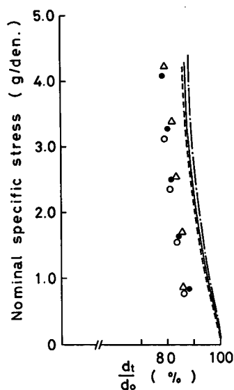
Fig. 3.42. Calculated and experimental values of diameter change by tensions of 3-ply cord 2-yarn strand at various surface helix angles,
