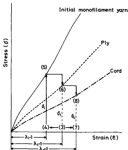
Fig. 4.2. Procedure of calculation of stress-strain curve of cord of single-yarn strand from the initial monofilament yarn stress-strain curve.
