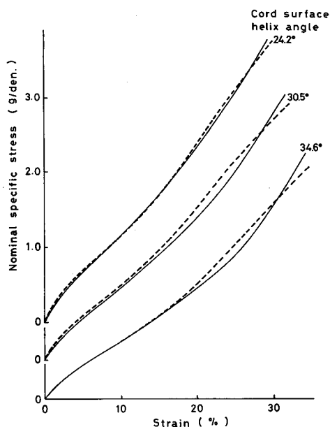
Fig. 4.14. Calculated and experimental stress-strain curves of 3-ply cord 2-yarn strand at various degrees of twisting. solid line; experimental, broken line; calculated.
