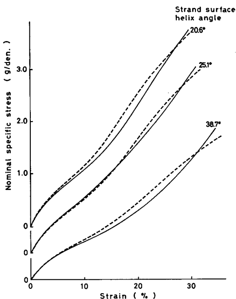
Fig. 4.10. Calculated and experimental stress-strain curves of 7-yarn strand at various degrees of twisting. solid line; experimental, broken line; calculated.
