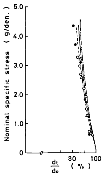
Fig. 3.41. Calculated and experimental values of diameter change by tensions of 2-ply cord 2-yarn strand at various surface helix angles.
