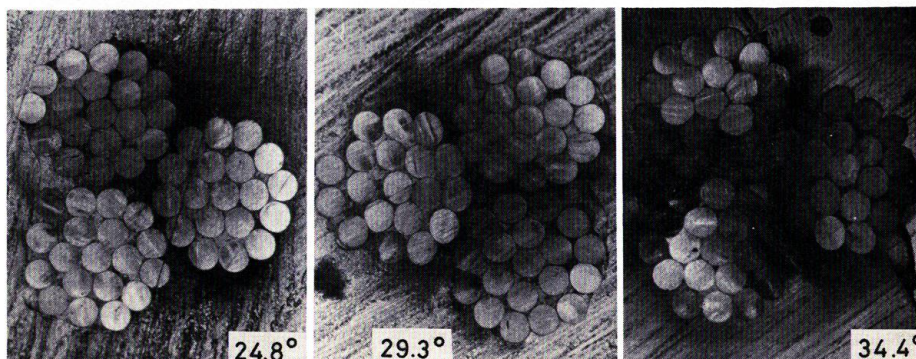
Fig. 3.36. Cross sections of 3-ply cord 19-yarn strand at various surface helix angles.
