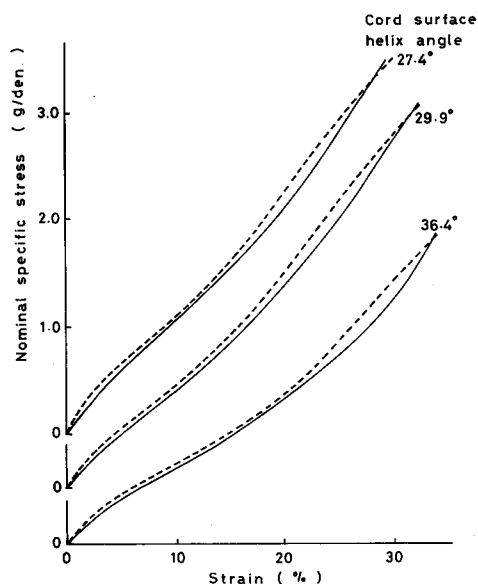
Fig. 4.17. Calculated and experimental stress-strain curves of 3-ply cord 7-yarn strand at various degrees of twisting. solid line; experimental, broken line; calculated.
