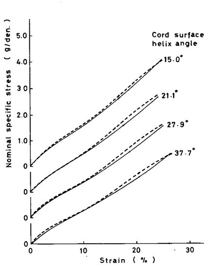
Fig. 4.4. Calculated and experimental stress-strain curves of 2-ply cord single-yarn strand of 30 turns per 6 in. lower twist at various degrees of twisting. solid line; experimental, broken line; calculated.
