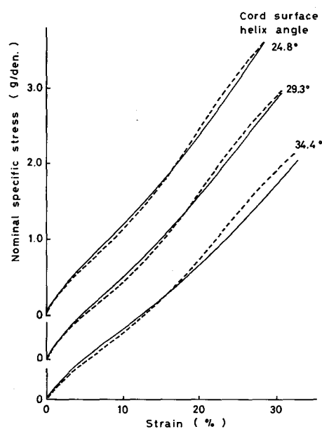
Fig. 4.19. Calculated and experimental stress-strain curves of 3-ply cord 19-yarn strand at various degrees of twisting. solid line; experimental, broken line; calculated
