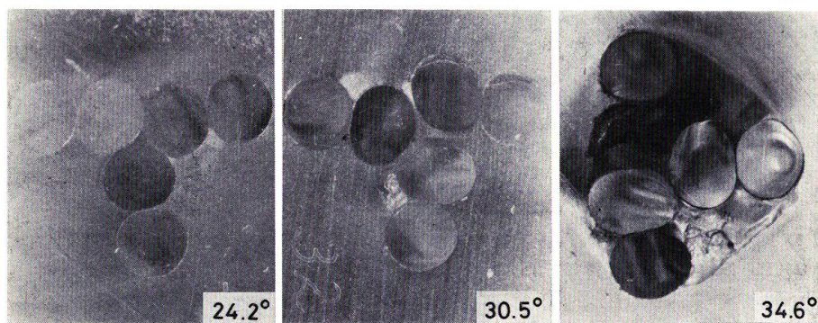
Fig. 3.30. Corss sections of 3-play cord 2-yarn strand at various surface helix angles.
