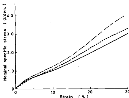
Fig. 5.2. Comparison between calculated curve of the present study and calculated using Treloar's formula with experimental result for 3-ply cord single yarn strand at 40.9^\circ surface helix angle.
