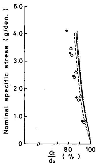
Fig. 3.43. Calculated and experimental values of diameter change by tensions 2-ply cord 3-yarn strand at various surface helix angles. \Delta ; experimental, ----; calculated, for 24.2^\circ surface helix angle, \bullet ; experimental, —; calculated, for 29.1^\circ surface helix angle, \circ ; experimental, ----; calculated, for 34.5^\circ surface helix angle.
