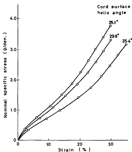
Fig. 3.25. Stress-strain curves of 2-ply cord 7-yarn strand at various degrees of twisting.
