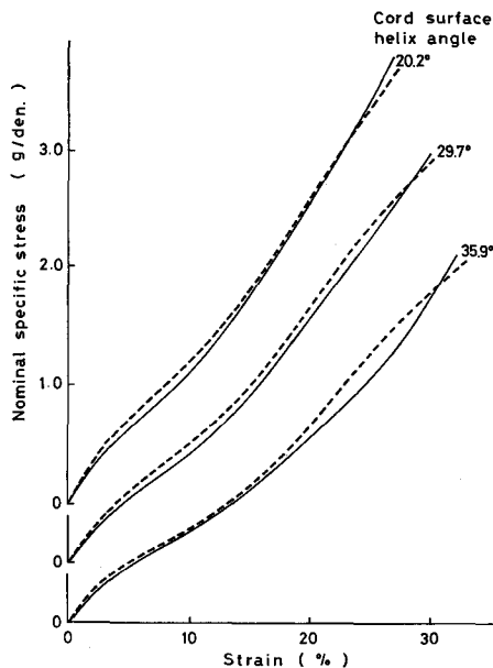
Fig. 4.12. Calculated and experimental stress-strain curves of 2-ply cord 2-yarn strand at various degrees of twisting. solid line; experimental, broken line; calculated.
