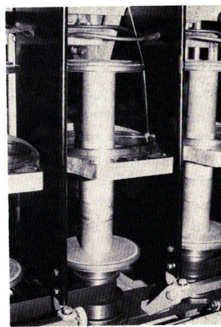
Fig. 3.4. Ring traveller and rotating bobbin.
