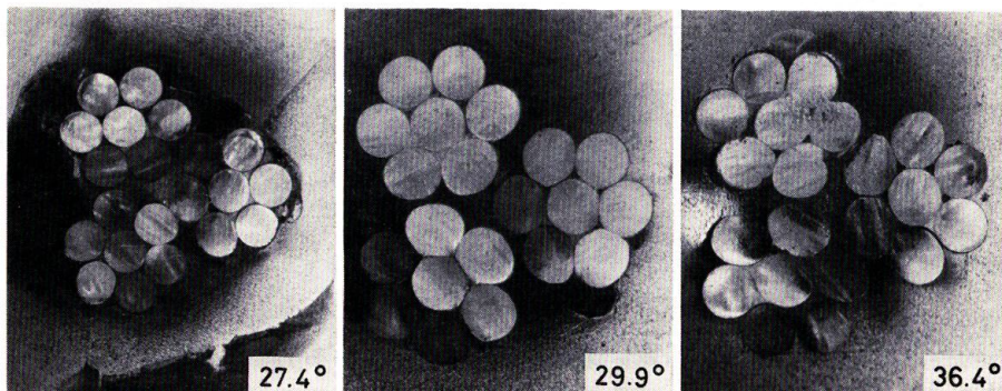
Fig. 3.34. Cross sections of 3-ply cord 7-yarn strand at various surface helix angles.
