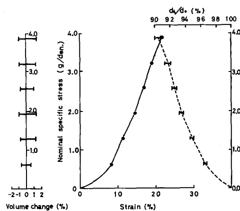
Fig. 5.1. Monofilament yarn diameter and volume change by tension.
