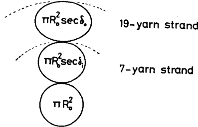
Fig. 4.1. Cross section area in individual monofilament yarn in the strand.
