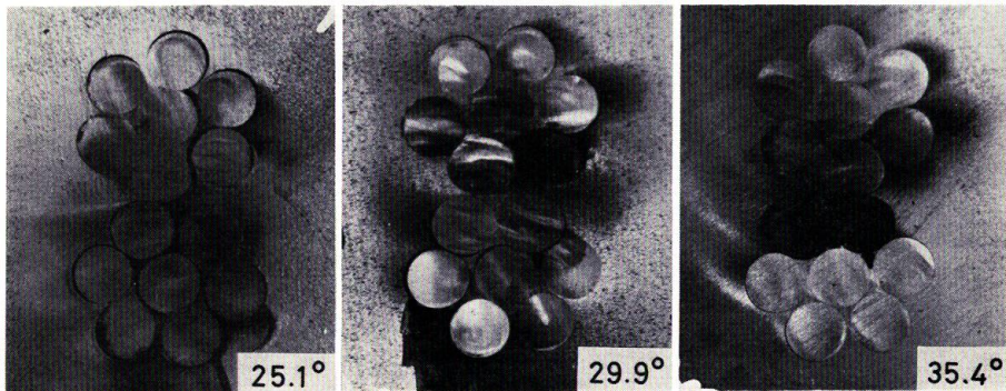
Fig. 3.33. Cross sections of 2-ply cord 7-yarn strand at various surface helix angles.
