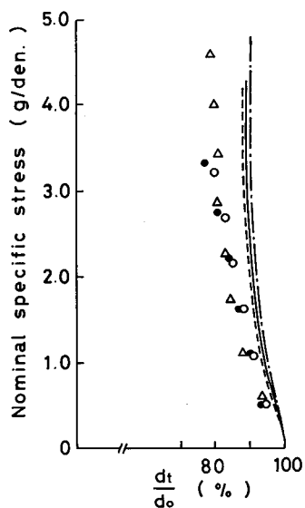
Fig. 3.44. Calculated and experimental values of diameter change by tensions of 3-ply cord 3-yarn strand at various surface helix angles, \Delta ; experimental, ----; calculated, for 26.2^\circ surface helix angle, \bullet ; experimental, —; calculated, for 29.3^\circ surface helix angle, \circ ; experimental, ----; calculated, for 31.9^\circ surface helix angle.
