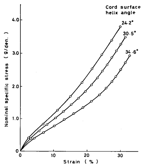
Fig. 3.22. Stress-strain curves of 3-ply cord 2-yarn strand at various degrees of twisting.
