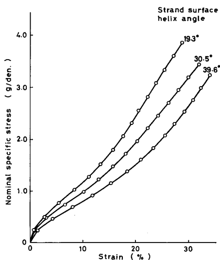
Fig. 3.17. Stress-strain curves of 2-yarn strand at various degrees of twisting.
