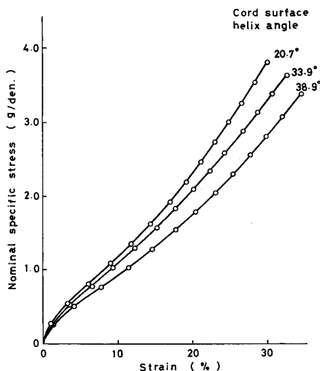
Fig. 3.27. Stress-strain curves of 2-ply cord 19-yarn strand at various degrees of twisting.
