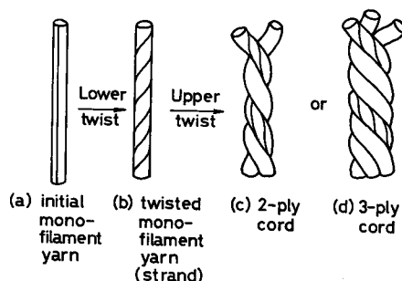
Fig. 2.1. Constructions of 2-ply and 3-ply cord single yarn strand.
