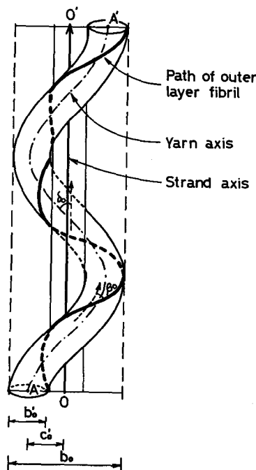
Fig. 2.8. Geometry of monofilament yarn as ply in the strand.
