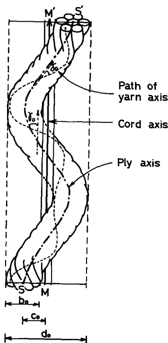
Fig. 2.7. Geometry of strand as ply in the cord.
