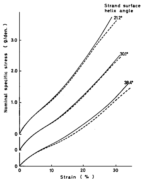
Fig. 4.11. Calculated and experimental stress-strain curves of 19-yarn strand at various degrees of twisting. solid line; experimental, broken line; calculated.
