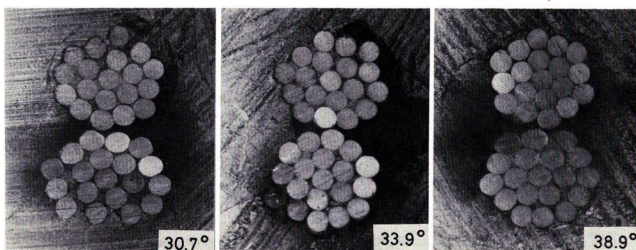
Fig. 3.35. Cross sections of 2-ply cord 19-yarn strand at various surface helix angles.
