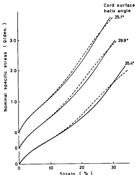
Fig. 4.16. Calculated and experimental stress-strain curves of 2-ply cord 7-yarn strand at various degrees of twisting. solid line; experimental, broken line; calculated.
