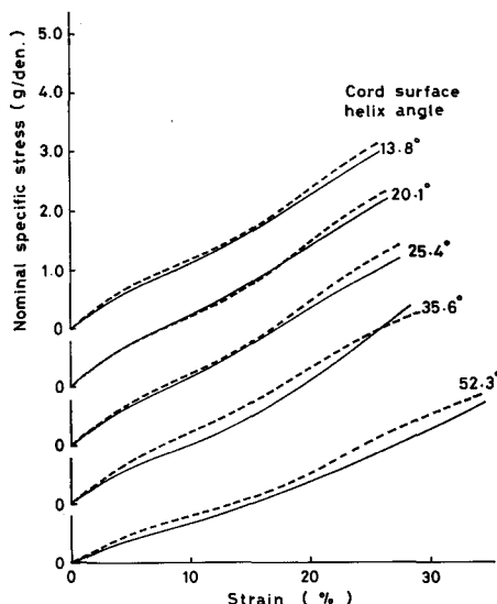
Fig. 4.3. Calculated and experimental stress-strain curves of 2-ply cord single yarn strand of 50 turns per 6 in. lower twist at various degrees of twisting. solid line; experimental, broken line; calculated.
