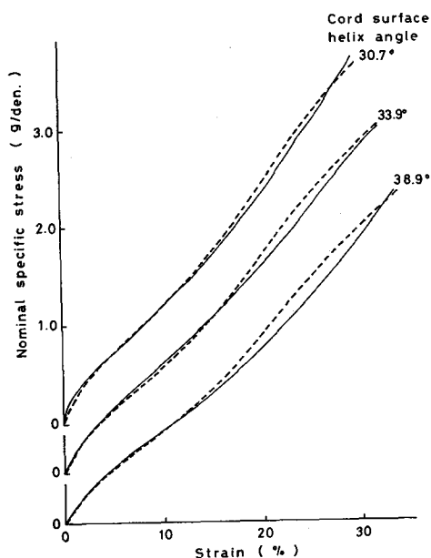
Fig. 4.18. Calculated and experimental stress-strain curves of 2-ply cord 19-yarn strand at various degrees of twisting. solid line; experimental, broken line; calculated.
