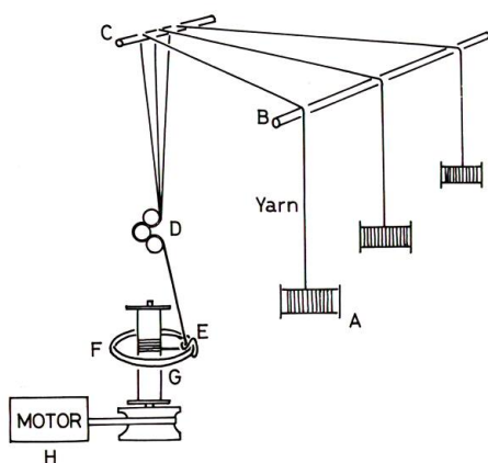
Fig. 3.1. Schematic diagram of ring traveller type twisting machine.
