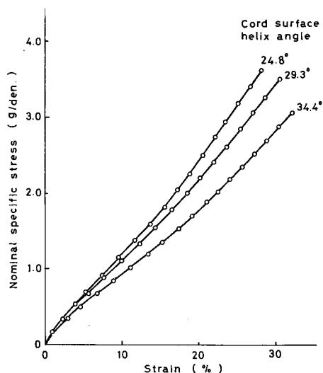
Fig. 3.28. Stress-strain curves of 3-ply cord 19-yarn strand at various degrees of twisting.
