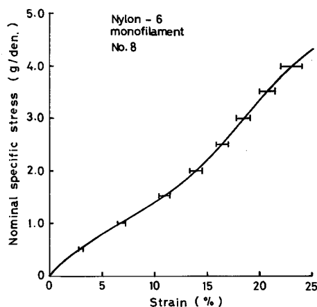
Fig. 3.16. Stress-strain curve of Nylon-6 monofilament No. 8.
