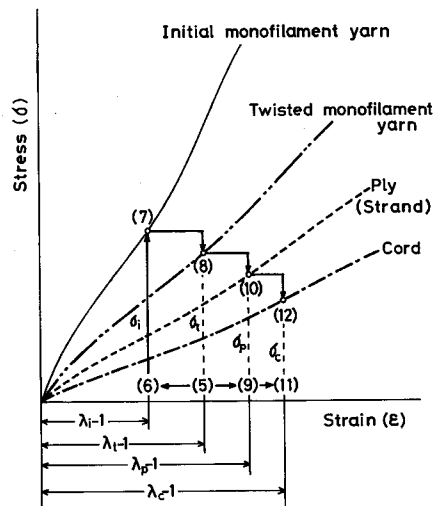
Fig. 4.7. Procedure of calculation of the stress-strain curve of cord of multiply-yarn strand from the initial monofilament yarn stress-strain curve.
