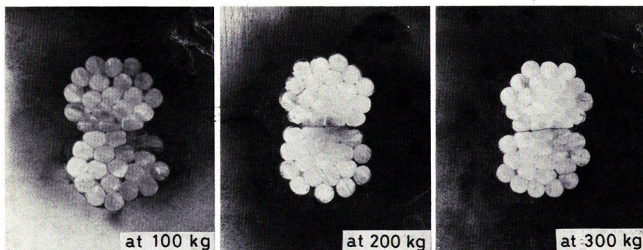
Fig. 3.38. Cross sections of 2-ply cord 19-yarn strand at various tensions.
