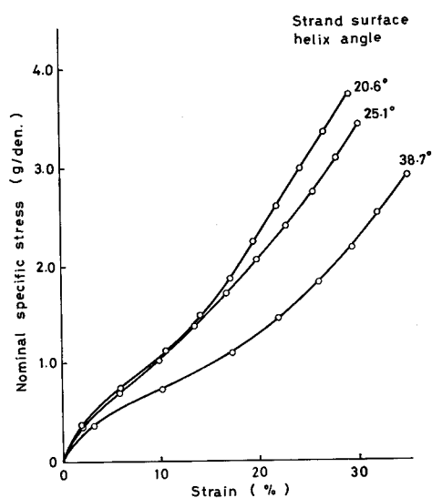
Fig. 3.19. Stress-strain curves of 7-yarn strand at various degrees of twisting.
