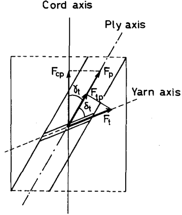
Fig. 2.9. Axial force acting in the cord of multiply-yarn strand.
