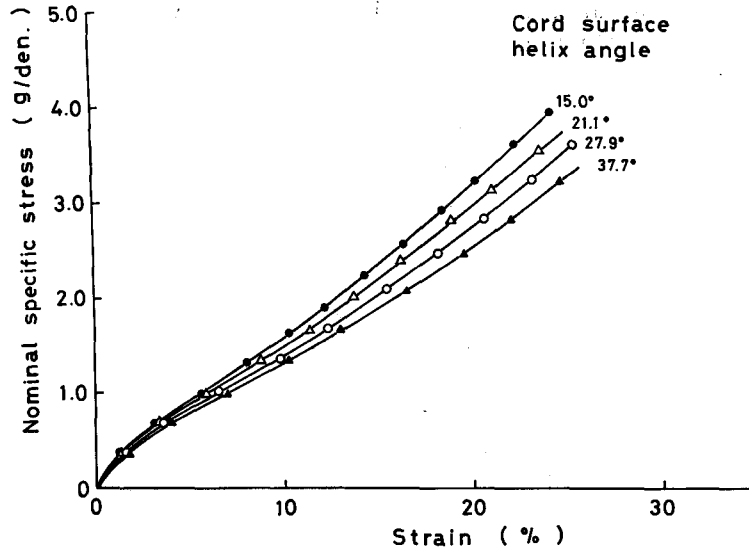
Fig. 3.8. Stress-strain curves of 2-ply cord single-yarn strand of 30 turns per 6 in. lower twist at various degrees of twisting.
