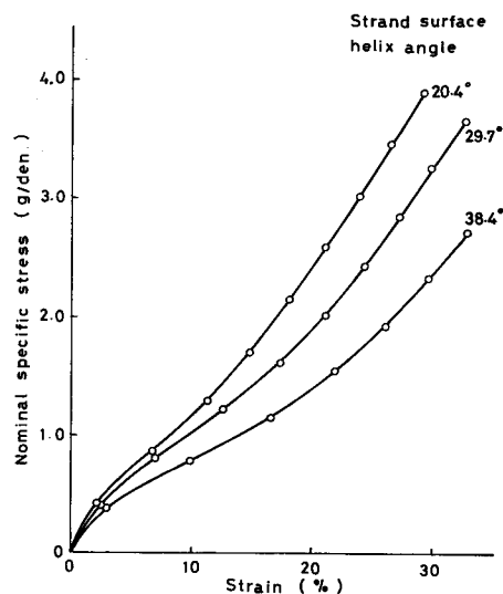
Fig. 3.18. Stress-strain curves of 3-yarn strand at various degrees of twisting.
