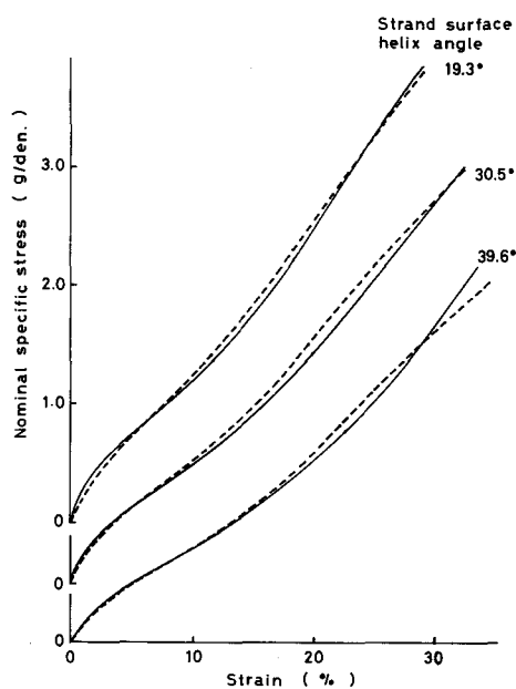
Fig. 4.8. Calculated and experimental stress-strain curves of 2-yarn strand at various degrees of twisting. solid line; experimental, broken line; calculated
