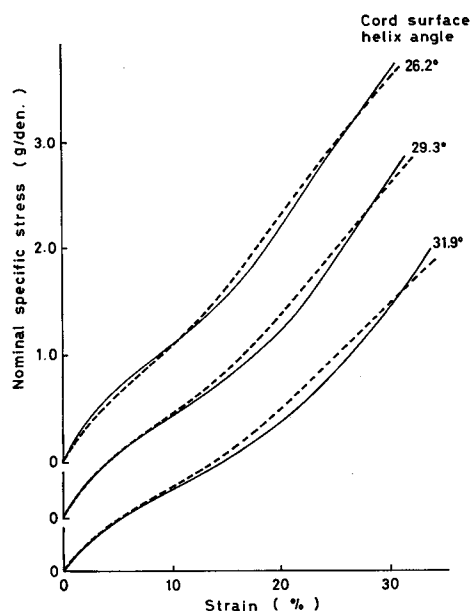
Fig. 4.15. Calculated and experimental stress-strain curves of 3-ply cord 3-yarn strand at various degrees of twisting. solid line; experimental, broken line; calculated.
