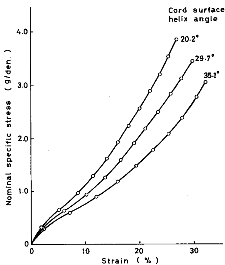
Fig. 3.21. Stress-strain curves of 2-ply cord 2-yarn strand at various degrees of twisting.
