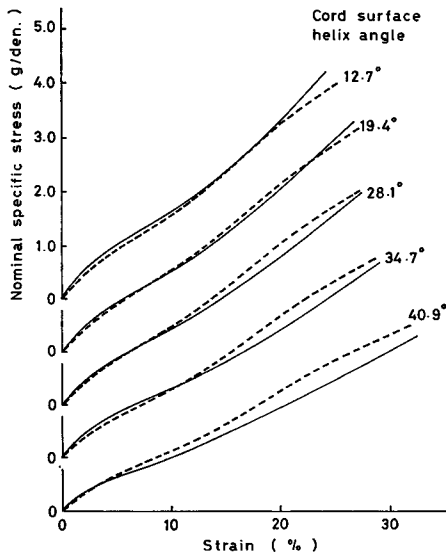
Fig. 4.6. Calculated and experimental stress-strain curves of 3-ply cord single yarn strand of 30 turns per 6 in. lower twist at various degrees of twisting. solid line; experimental, broken line; calculated.
