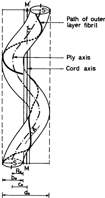
Fig. 2.5. Geometry of monofilament yarn as ply in the cord.
