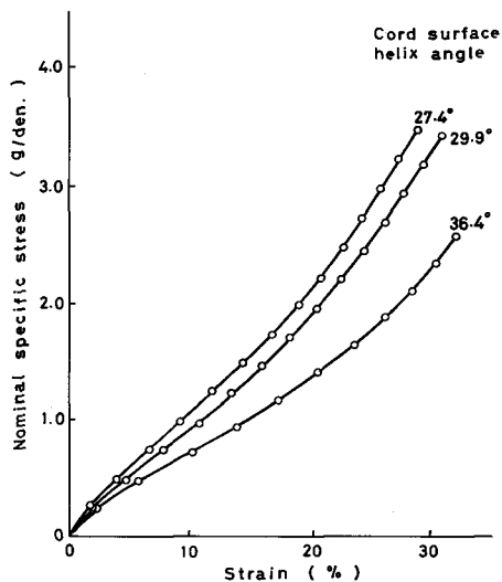
Fig. 3.26. Stress-strain curves of 3-ply cord 7-yarn strand at various degrees of twisting.
