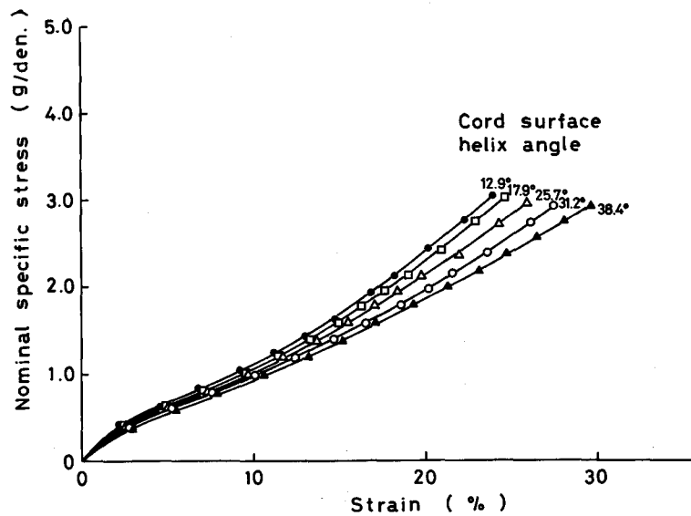
Fig. 3.9. Stress-strain curves of 3-ply cord single-yarn strand of 50 turns per 6 in. lower twist at various degrees of twisting.
