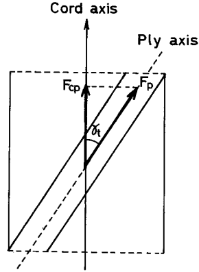
Fig. 2.6. Axial force acting in the cord of single-yarn strand.
