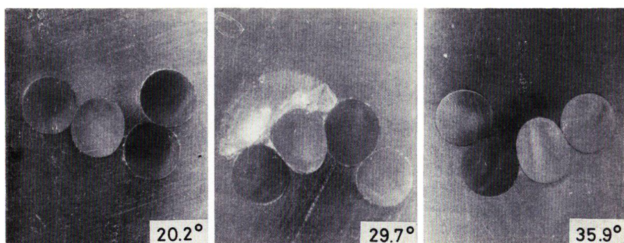
Fig. 3.29. Cross sections of 2-ply cord 2-yarn strand at various surface helix angles.
