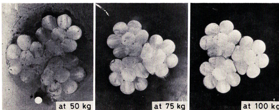
Fig. 3.37. Cross sections of 3-ply cord 7-yarn strand at various tensions.
