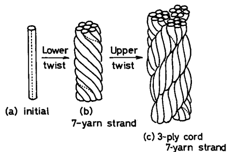
Fig. 2.2 Construction of 3-ply cord 7-yarn strand.
