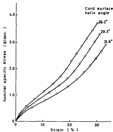
Fig. 3.24. Stress-strain curves of 3-ply cord 3-yarn strand at various degrees of twisting.
