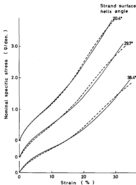
Fig. 4.9. Calculated and experimental stress-strain curves of 3-yarn strand at various degrees of twisting. solid line; experimental, broken line; calculated.
