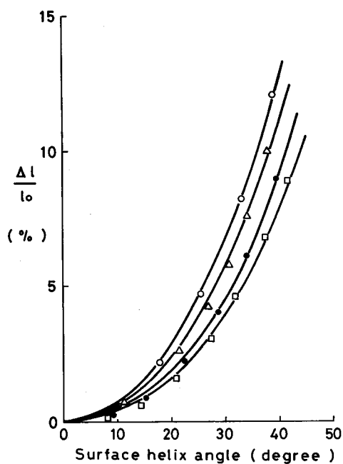
Fig. 3.46. Calculated and experimental values of strand retraction ratio. \square ; 2-yarn strand, \bullet ; 3-yarn strand, \Delta ; 7-yarn strand, \circ ; 19-yarn strand, solid-line: calculated values.
