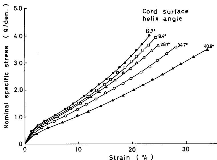
Fig. 3.10. Stress-strain curves of 3-ply cord single-yarn strand of 30 turns per 6 in. lower twist at various degrees of twisting.
